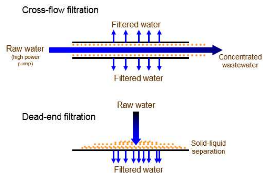
Fig. 3 Cross-flow filtration and dead-end
