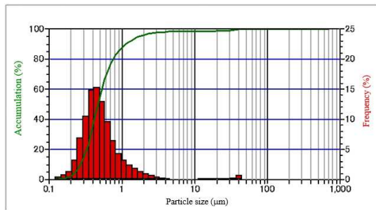
Fig. 2 Particle sizes of silicon fragments contained in the wastewater from the dicer.
