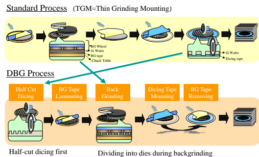
Fig.2 DBG process flow
